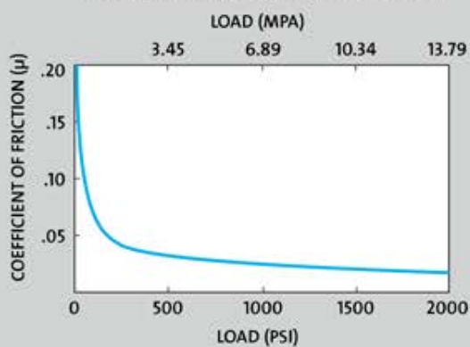
FIGURE 5: COEFFICIENT OF FRICTION VS. LOAD
