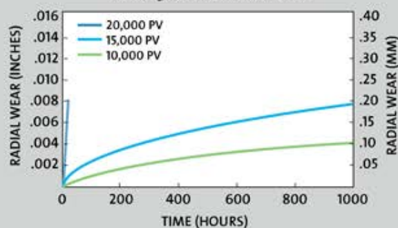
FIGURE 3: RADIAL WEAR VS. TIME
