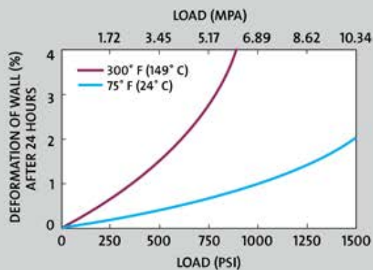
FIGURE 4: DEFORMATION VS. LOAD (RULON® LR)
