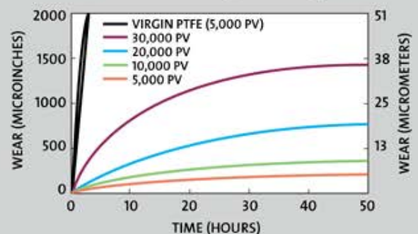
FIGURE 10: WEAR VS. TIME AT VARIOUS PV'S (RULON® 641)
