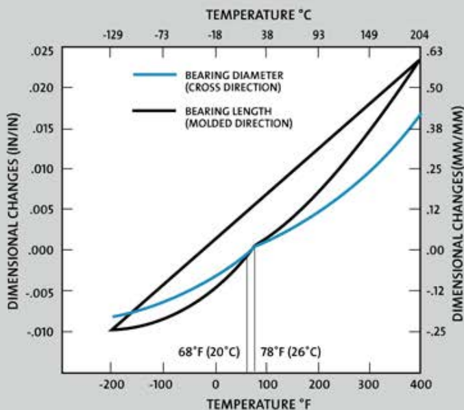
FIGURE 11: THERMAL EXPANSION OF RULON® 641
